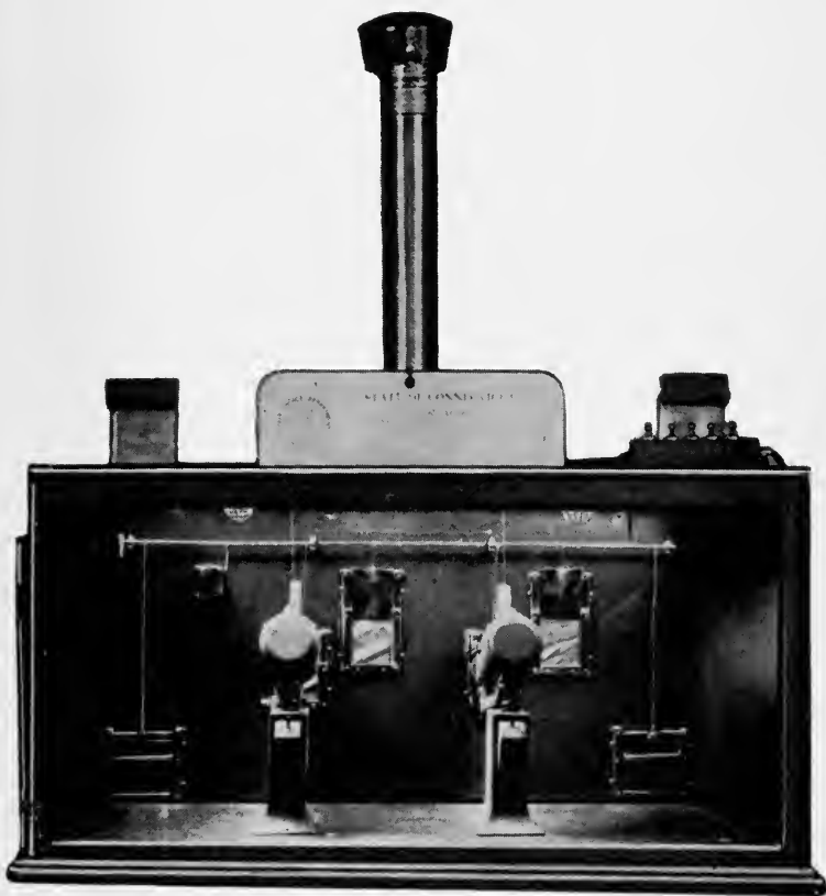
FIG. 1. Complete model of projection room (width about two feet) viewed from the rear.
